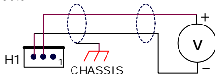
0-5VDC Input Diagram
