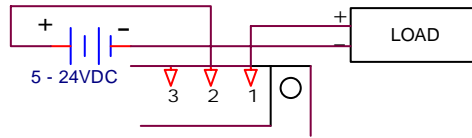
CONFIGURED FOR SOURCING CURRENT
