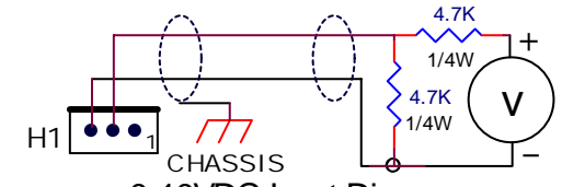
0-10VDC Input Diagram
