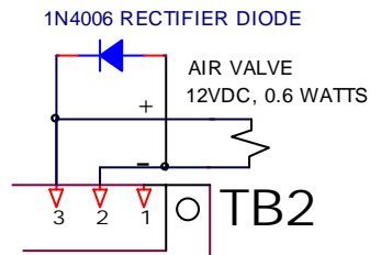
Typical relay or air valve wiring
